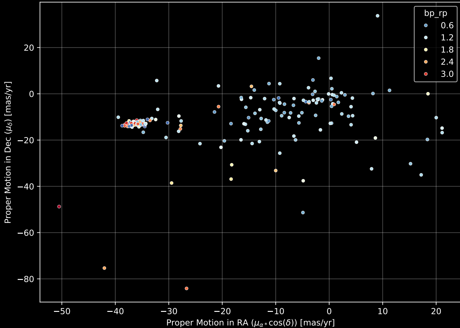
APOGEE DR17 Field: [K2_C5_206+32_btx] Proper Motion Diagram (n= 206)
