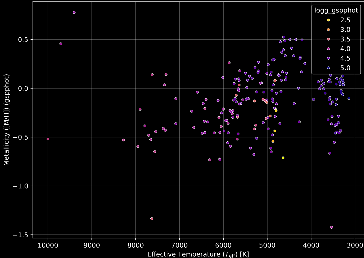
APOGEE DR17 Field: [K2_C5_206+32_btx] Stellar Population Parameters (n= 206)
